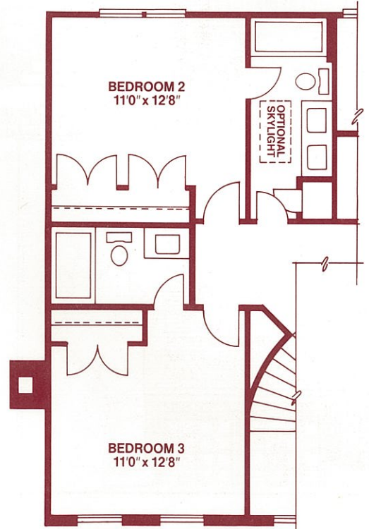
PARTIAL UPPER FLOOR PLAN / THIRD BATH OPTION
