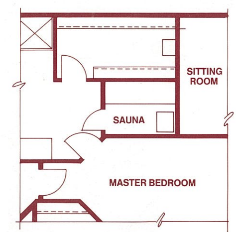
PARTIAL UPPER FLOOR PLAN / SAUNA OPTION
